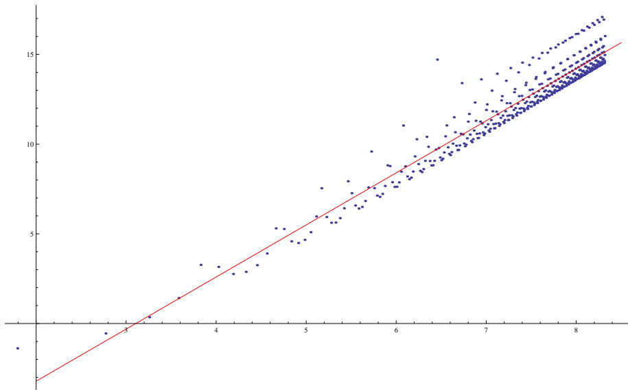
Figure 1b: The graph of -\log(|\varphi_e(3, N) - \varphi(3)|) against \log N in Example 5.1
